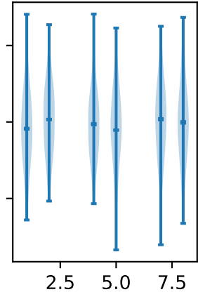
Custom violinplot 3
